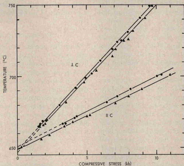
Fig. 6. Temperature of the \alpha - \beta transition at a constant confining pressure of 3 kb as a function of compressive stress \perp C (run 602) and \parallel C (run 603). The transition \beta \rightarrow \alpha (increasing stress) is denoted by triangles, whereas \alpha \rightarrow \beta (decreasing stress) is denoted by circles. See Table 2 for least-squares values of slope and intercept for these runs.
